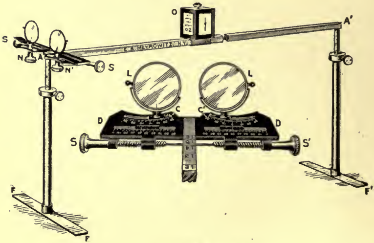
FIG. 210.—Optometer of the author.
